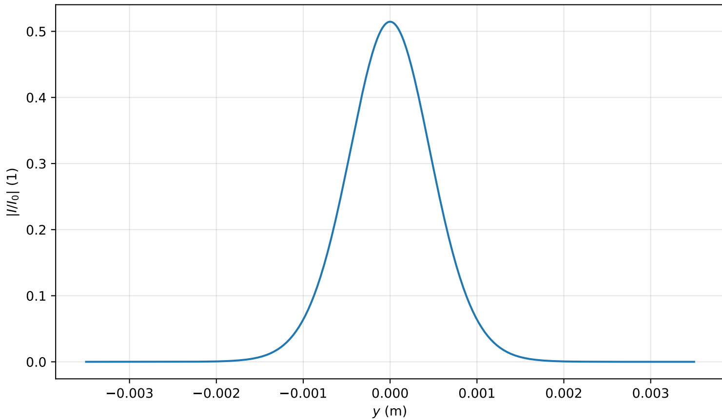
Intensity profile I(x=0, y, z=2.548)/I_0 , P_{in}=0.3P_{cr} , artificial time
